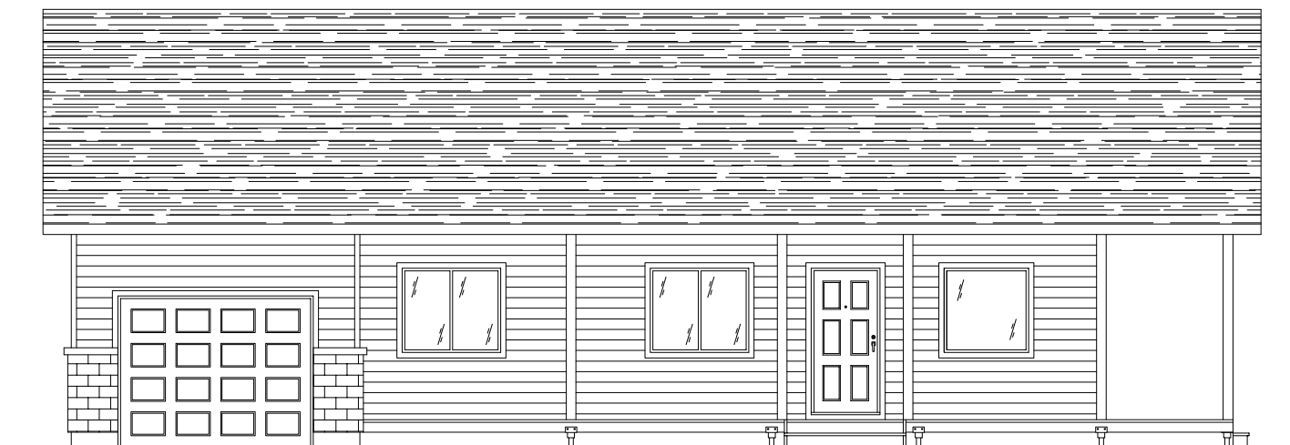
FRONT ELEVATION
