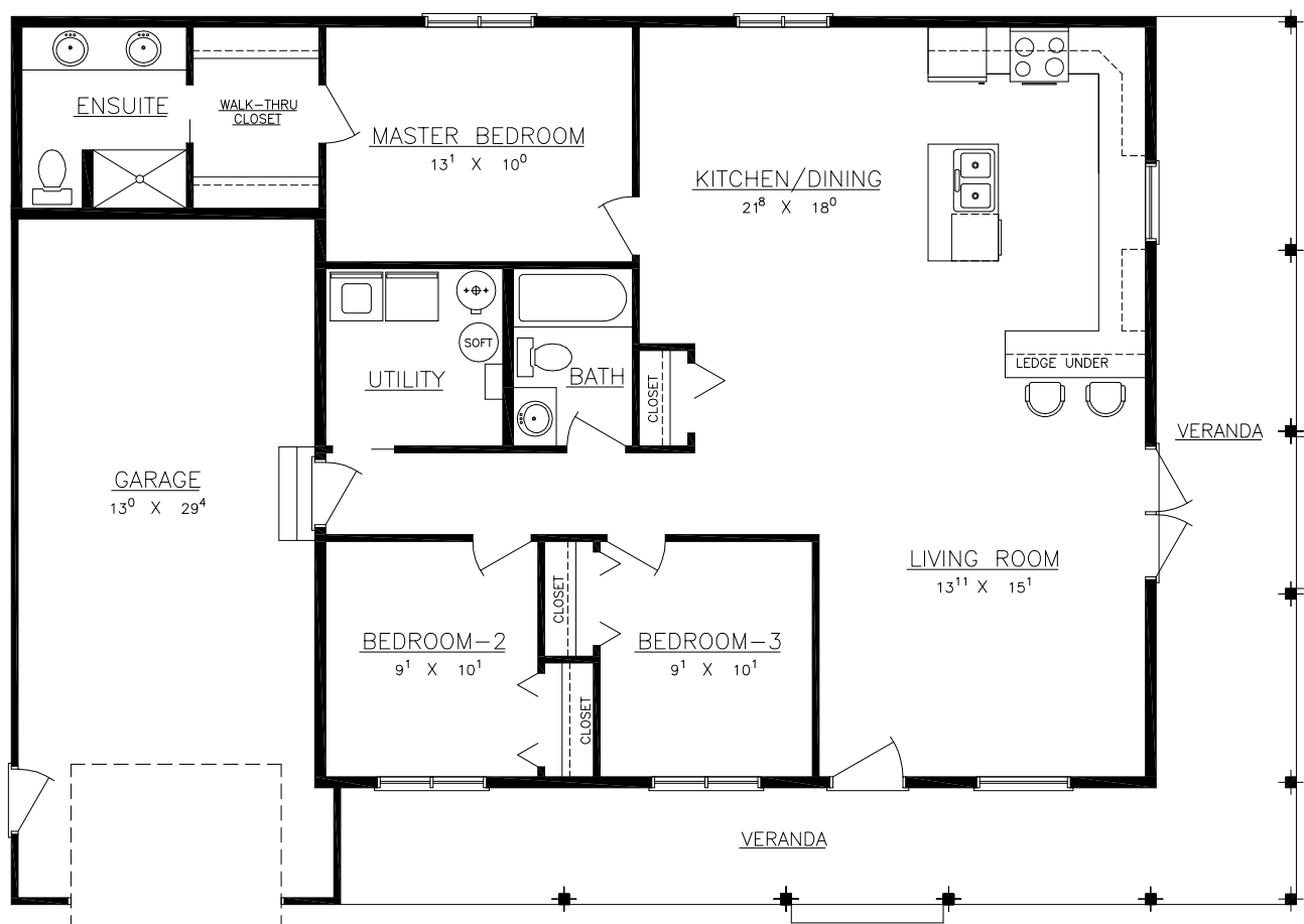
FLOOR PLAN
